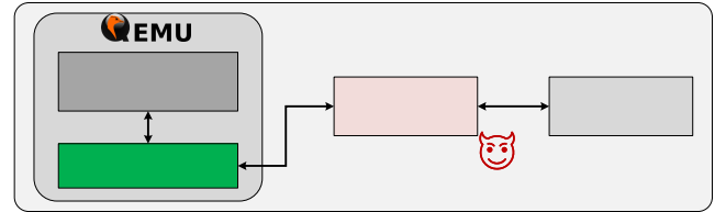
Figure 4: Reproducing BLE host vulnerabilities with PERRY.
