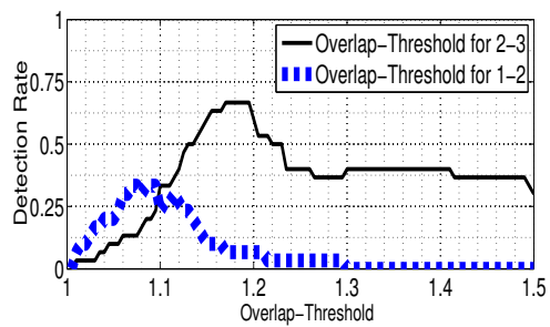
Figure 14: Deriving Overlap-threshold
