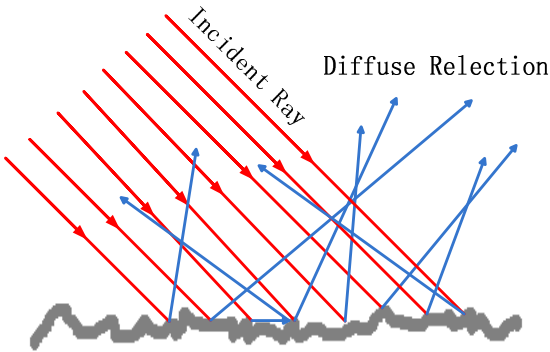
Figure 7: Diffuse Reflection
