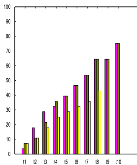
Fig. 7. Semi-supervised allocation without load balancing in hierarchical multiagent network. (i) Occupancy percentage of allocated agents; (ii) Mean geodesic distance between vertex pairs in the allocated agents; (iii) Mean geodesic eccentricity of allocated agents; (iv) Execution time of task.
