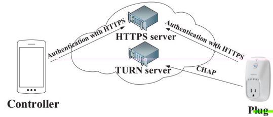
Fig. 12. Authentication phase.
