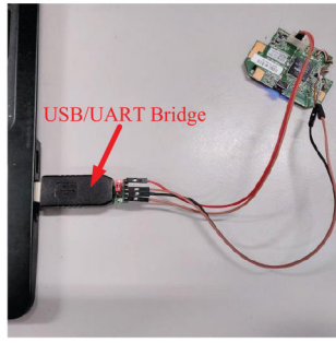
Fig. 9. Open a console of WeMo plug system by UART.
