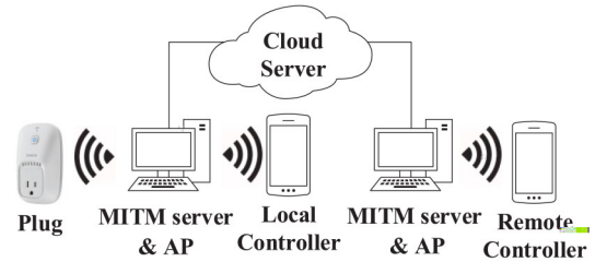
Fig. 7. NAT traffic collection.
