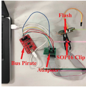
Fig. 4. Reading flash by bus pirate.
